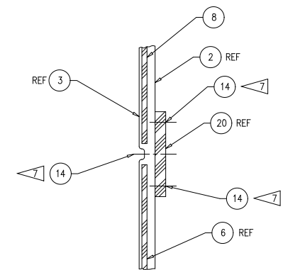
SECTION F-F SCALE: 2/1 2X
