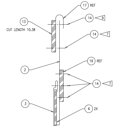
SECTION E-E SCALE: 2/1 2X
