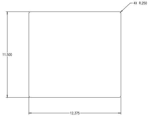
⑨ INSERT, FRONT 5 18
