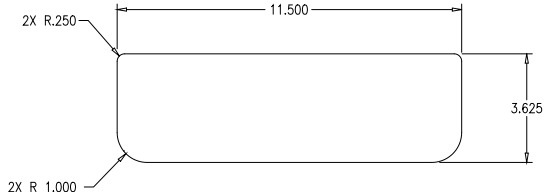
⑥ INSERT, BODY END 5 18 2X
